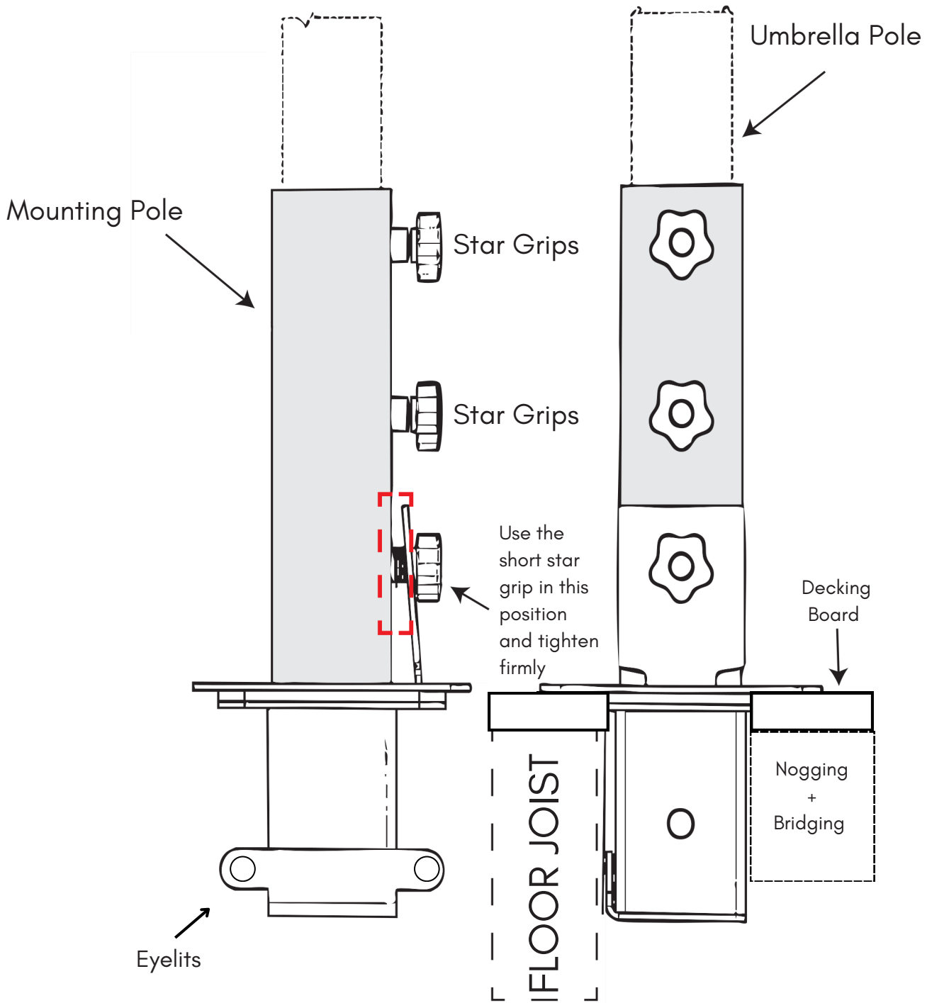
SIDE VIEW
